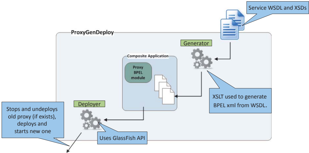
Figure 2. Architecture of ProxyGenDeploy.
