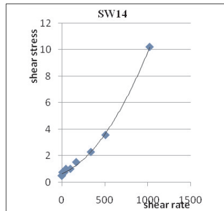
Fig. 21. Slick water SW14 (700 g/L)
