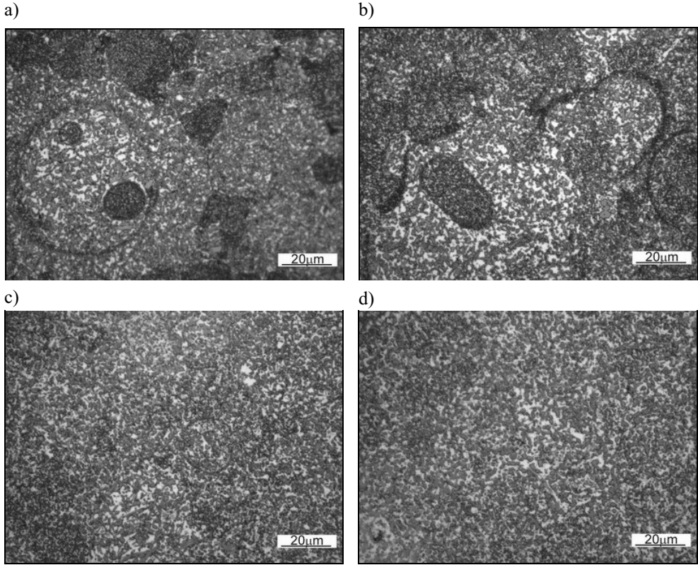
Fig. 5. Microstructures of materials obtained in closed-die hot compaction of Al_{17}Si_5Fe_3Cu_{1.1}Mg_{0.6}Zr powder. Transverse sections, after etching: a) temperature 400\text{ }^{\circ}C , punch unit pressure 50 MPa; b) 450\text{ }^{\circ}C , 150 MPa; c) 485\text{ }^{\circ}C , 150 MPa; d) 500\text{ }^{\circ}C , 150 MPa
