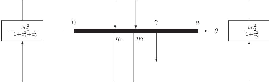
Fig. 5. Optimal feedback controller realization in the MISO case
