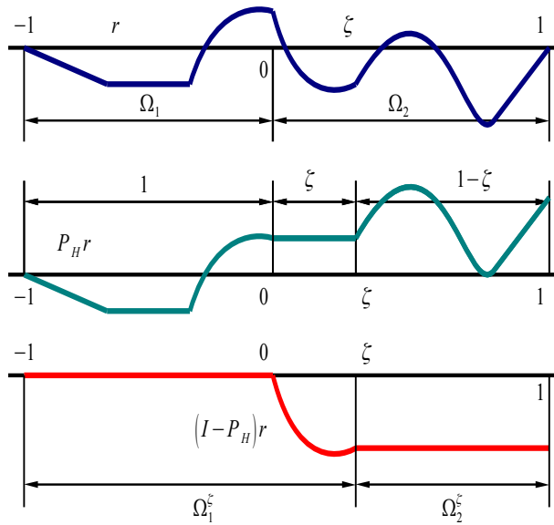
Fig. 2. Orthogonal decomposition
