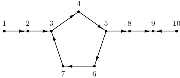
Fig. 4. A cycle-oriented cactus
