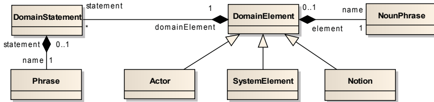
Figure 5. Abstract syntax of domain vocabulary elements.
