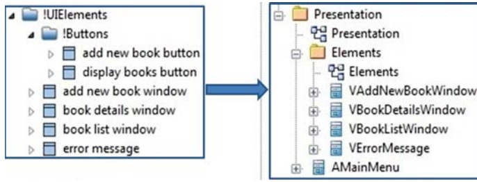
Figure 8. Generation of the view layer classes.
