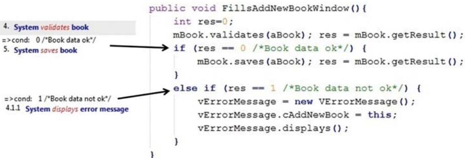
Figure 11. Dynamic code generated for condition sentences.
