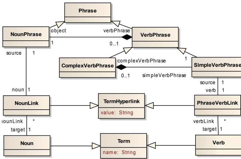
Figure 4. Abstract syntax of sentence phrases.
