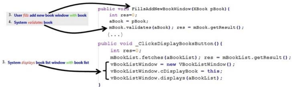
Figure 10. Dynamic code generated for SVO sentences.
