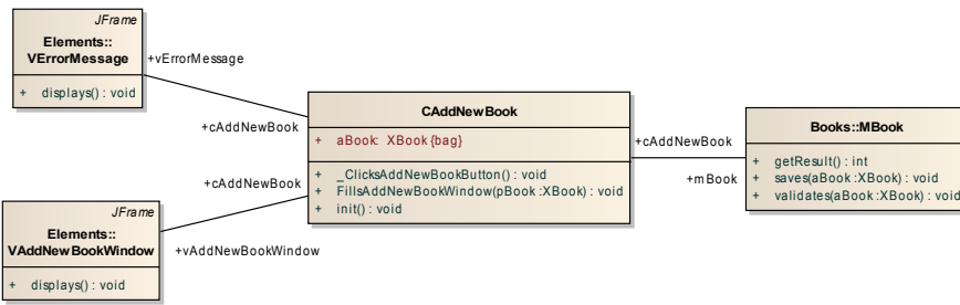
Figure 9. General structure of the generated code.
