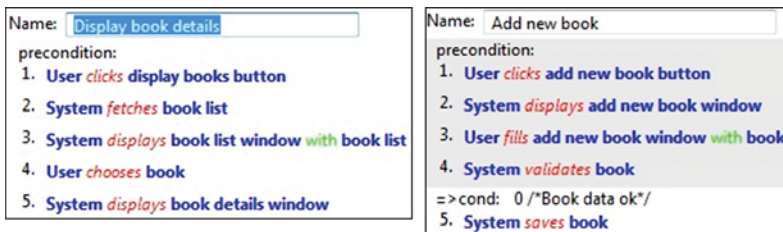
Figure 2. Concrete syntax for use case scenarios.
