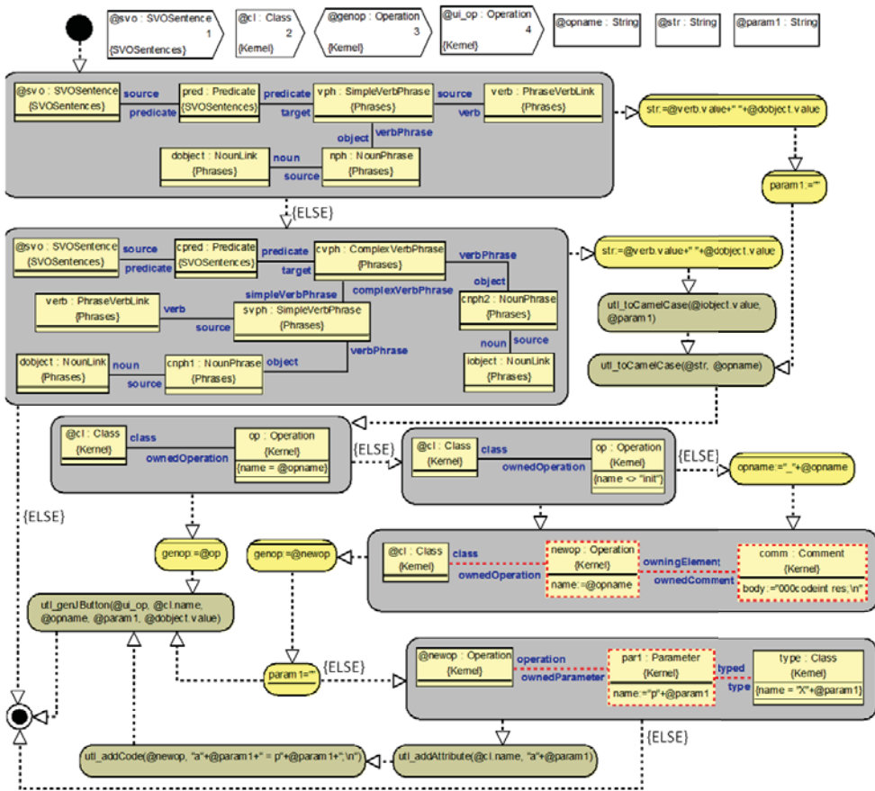
Figure 17. Actor-to-System sentence processing procedure.
