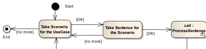
Figure 13. General algorithm for use case processing.
