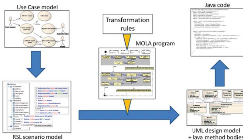
Figure 1. Overview of the translation process.
