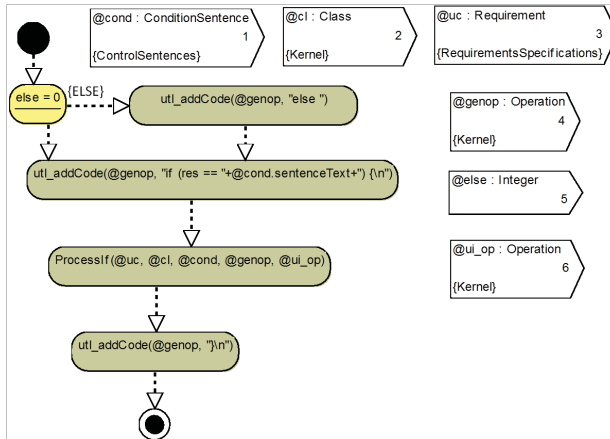
Figure 18. Condition sentence processing procedure.
