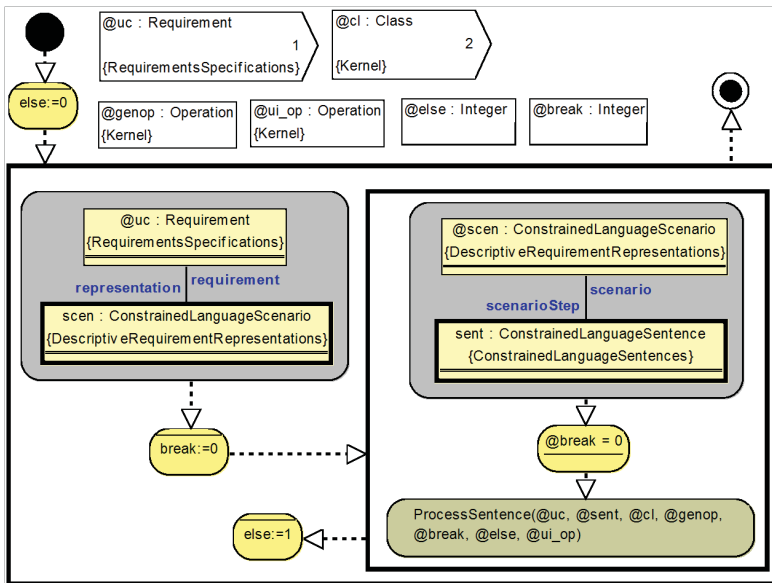
Figure 15. Main use case transformation procedure.
