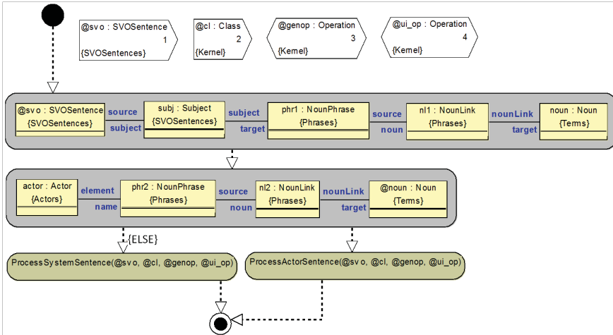
Figure 16. SVO sentence processing procedure.
