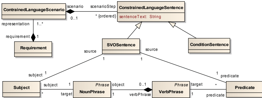
Figure 3. Abstract syntax of use case scenarios and sentences.
