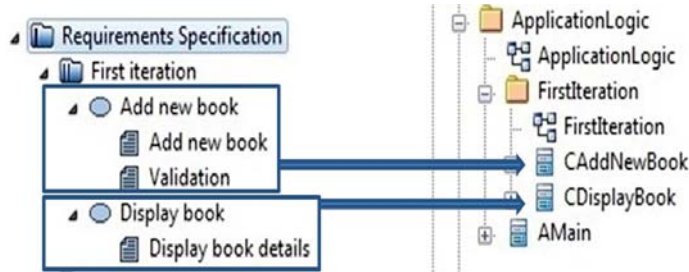
Figure 6. Generation of the controller/presenter layer classes.
