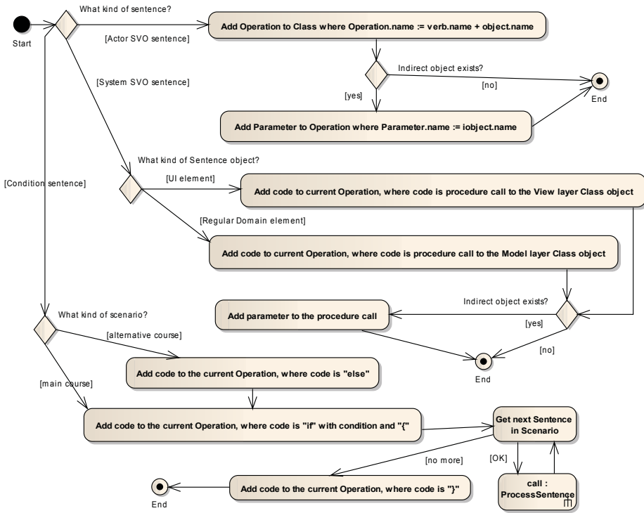
Figure 14. General algorithm for scenario sentence processing (ProcessSentence procedure).
