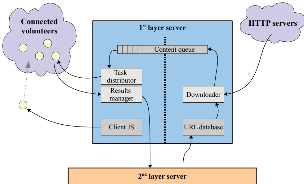
Figure 3. Processing performed by a first layer server.
