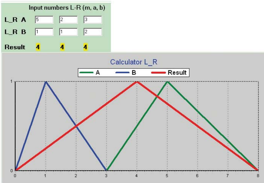
Figure 8. Solution of the equation A + X = C using L-R numbers.
