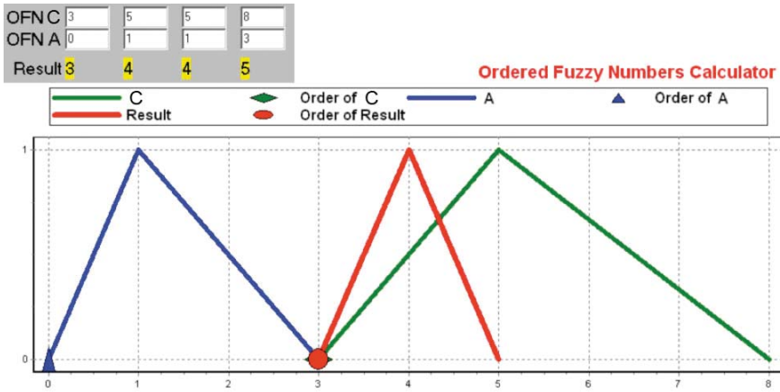
Figure 9. Results of C[3, 5, 5, 8] (positive order) - A[0, 1, 1, 3] (positive order).
