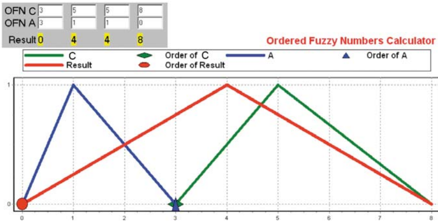
Figure 11. Result of C[3, 5, 5, 8] (negative order) - A[3, 1, 1, 0] (positive order).
