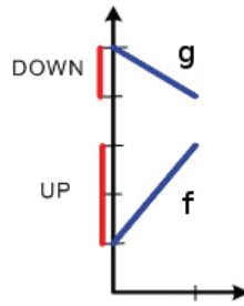
Figure 2. Ordered fuzzy number.
