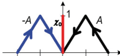
Figure 5. Opposite numbers and the real number.
