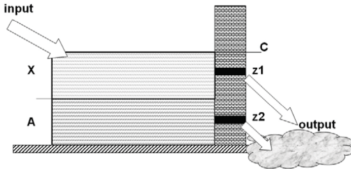
Figure 1. The diagram of water flow in the impounding basin.
