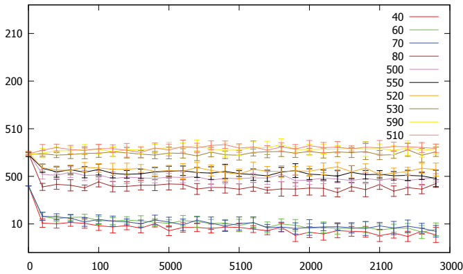
Figure 7. Influence of agent initial on EMAS agent count agentCount(step) .
