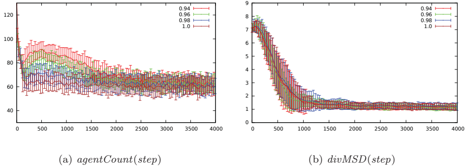
Figure 21. Influence of “good” fitness percentage on agent count and diversity.
