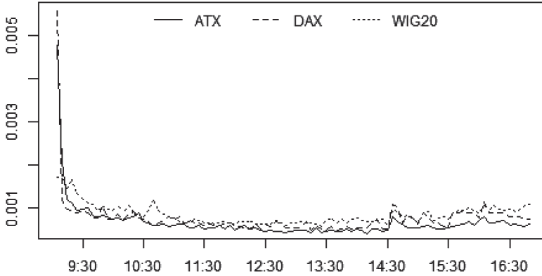
Figure 1. Cross-sectional standard deviations of 5-minute returns of ATX, DAX, and WIG20 during period of March 22, 2013 – July 31, 2014
