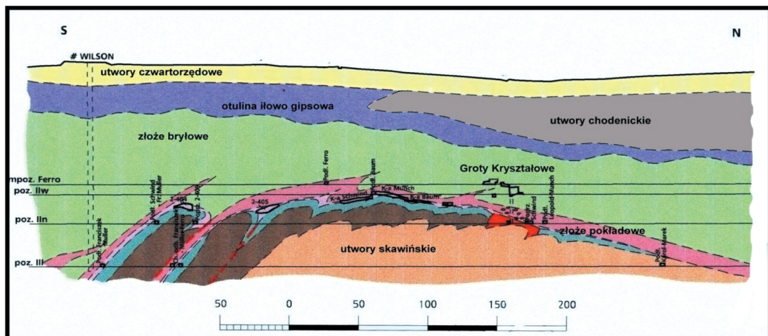
Fig. 1. Cross-section through the dome of the Crystal Grotto [3]
