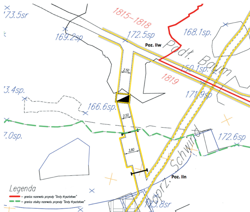
Fig. 6. Layout of the planned excavations
