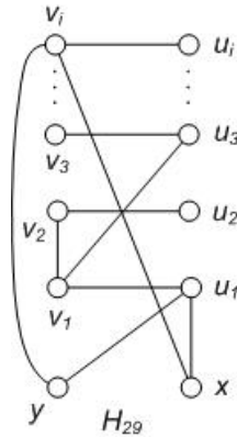
Fig. 18. v_i, \text{ for } i \geq 4, \text{ is adjacent to } x \text{ and } y
