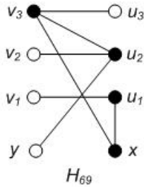
Fig. 38. The case k = 3
