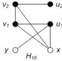
Fig. 8. The graph obtained from H_{10} by adding an edge
