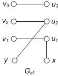
Fig. 37. The spanning forest for k = 3
