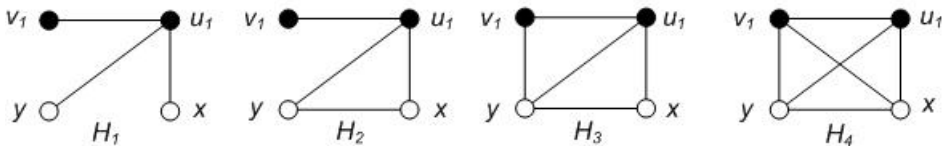
Fig. 2. The graphs for Case 1.1.
