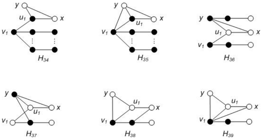
Fig. 24. The exhaustive cases
