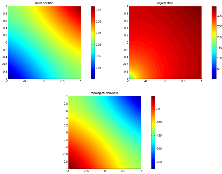
Fig. 1. Direct solution, adjoint state and topological derivative
