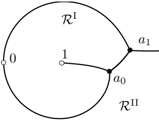
Fig. 3.2. (0.5, 1 - \hat{\epsilon}i, 1)
