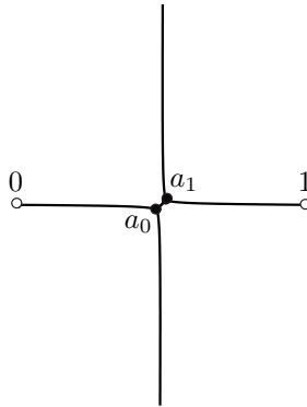
Fig. 3.8. (-\hat{\epsilon}i, 2, 1)
