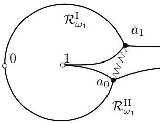
Fig. 3.1. (\alpha, \beta, \gamma) = (0.5, 1 + \epsilon - \hat{\epsilon}i, 1) in \omega_1
