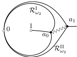
Fig. 3.3. (0.5, 1 - \epsilon - \hat{\epsilon}i, 1) in \omega_2
