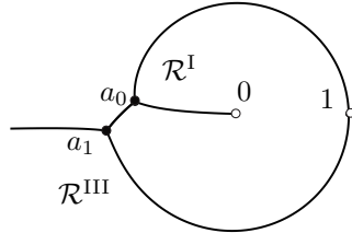
Fig. 3.5. (1 + \hat{\epsilon}i, 2, 1)
