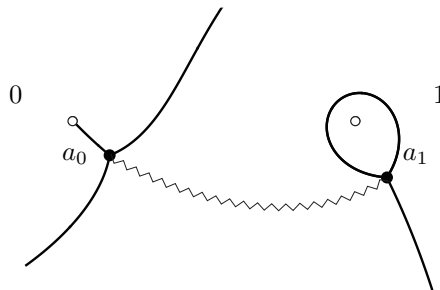
Fig. 3.10. (\alpha, \beta, \gamma) = (-0.5, 1.5 + \hat{\epsilon}i, 1)
