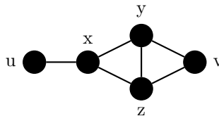
Fig. 1. The plane of graph G_1
