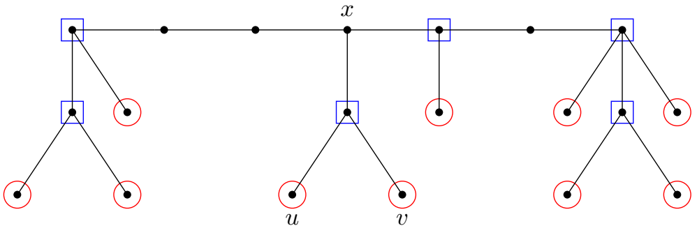
Fig. 5. An example of the tree which does not have disjoint (1, 1) -dset and (1, \bar{2}) -dset
