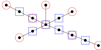
Fig. 4. The spider SP(1, 2, 4, 2, 3)
